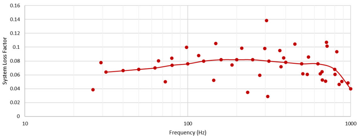
Decidamp CLS 50 on 5mm Steel Panel
