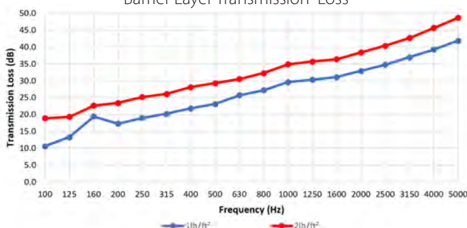
Barrier Layer Transmission Loss
