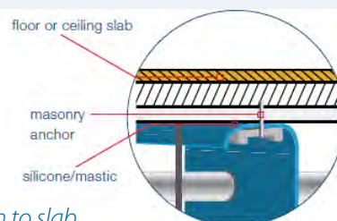
Installation to slab
