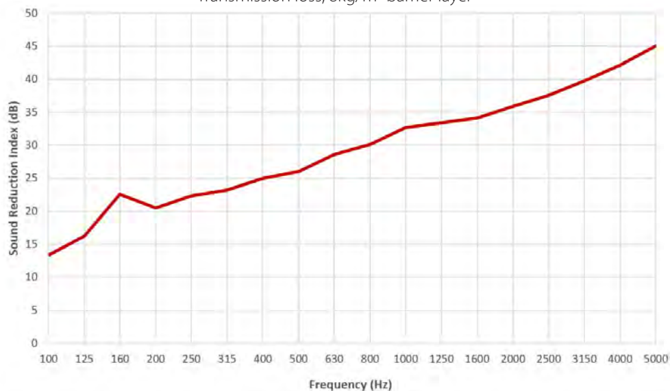
Transmission loss, 8kg/m 2 barrier layer
