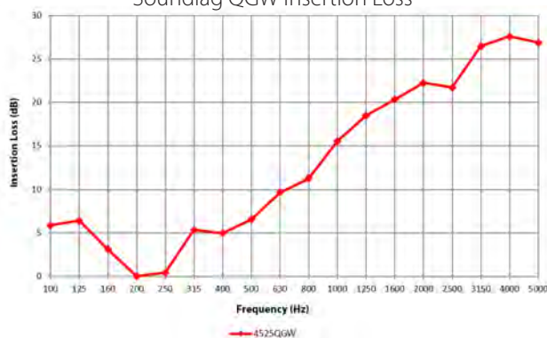
Soundlag QGW Insertion Loss
