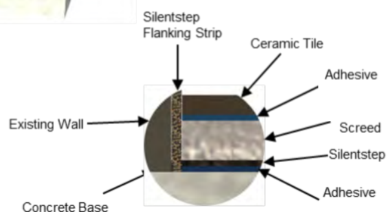
Flanking Strip Installation
